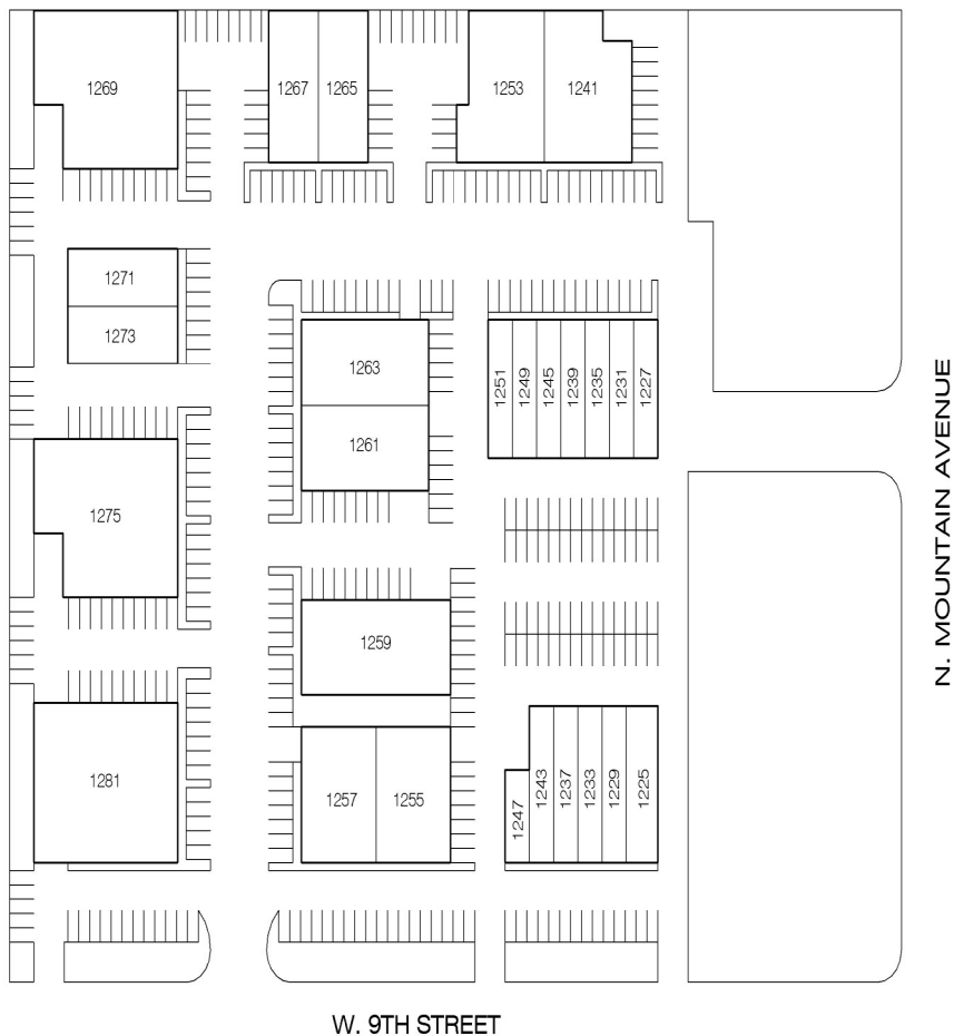
SITE PLAN - Mountain View Industrial Park, Upland
